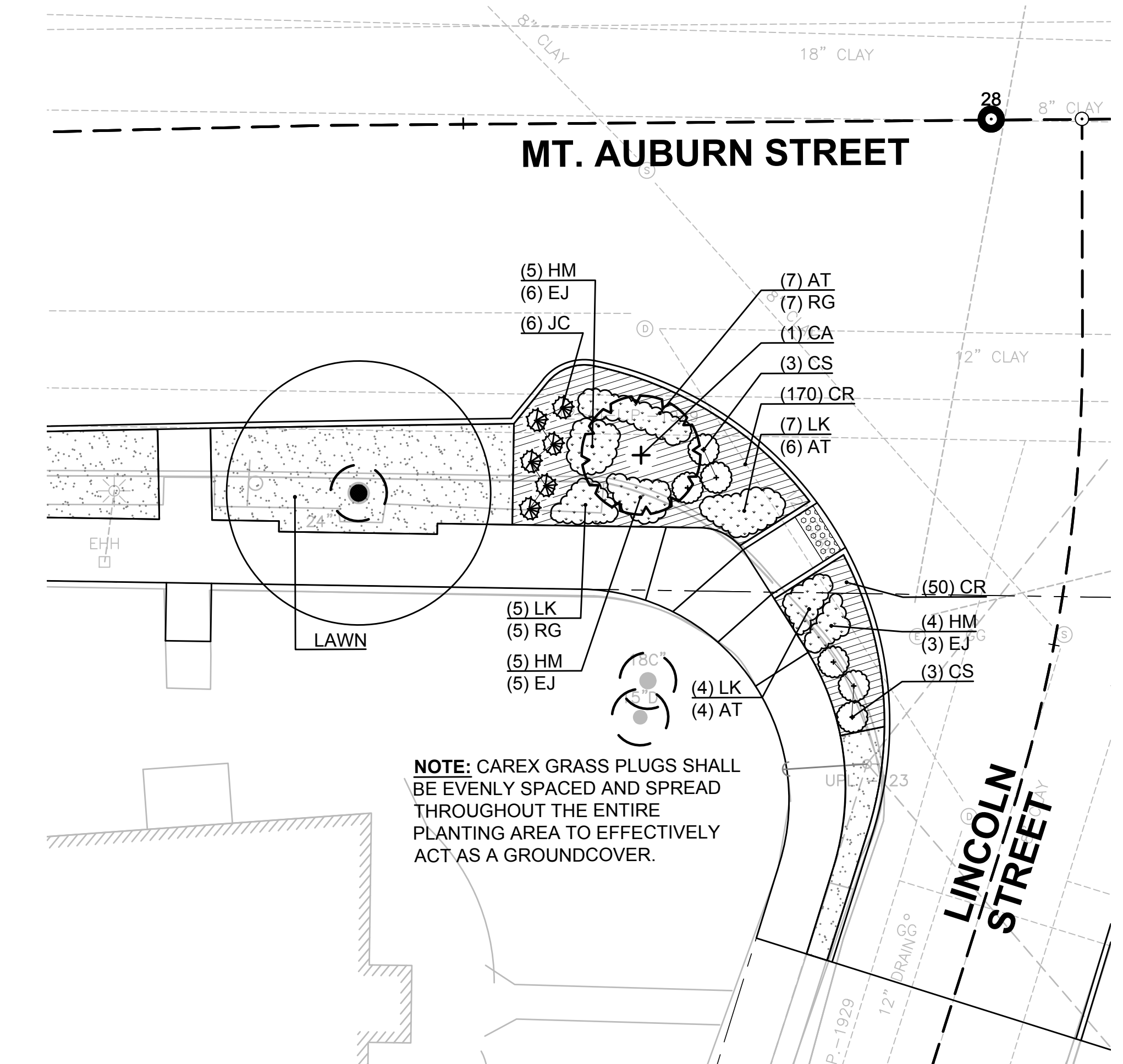
2 PLANTING AREA AT LINCOLN STREET & MT. AUBURN STREET INTERSECTION SCALE: 1"=10'-0"
